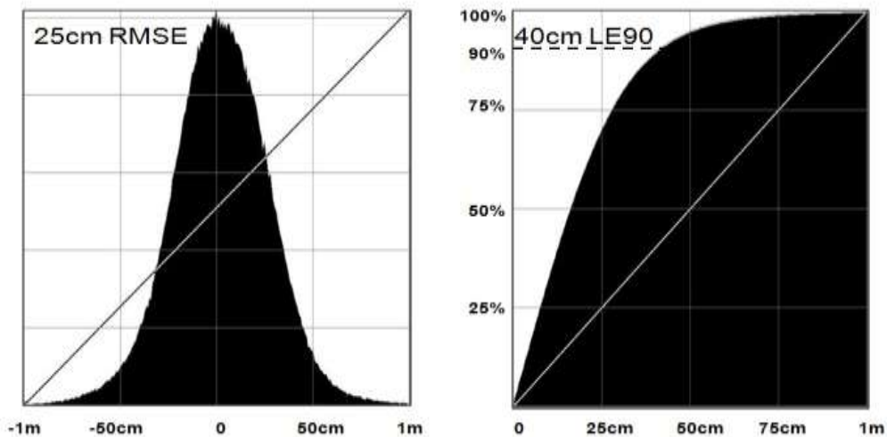
Figure 14. The elevation differences between the GeoEye-1 and LiDAR DEMs are shown in a standard histogram on the left and a cumulative histogram on the right. These histograms were created in ERMMapper. If we assume that the LiDAR DEM is perfect, the GeoEye-1 DEM elevations have an RMSE of 25cm. Ninety percent of the stereo GeoEye-1 elevations are within 40cm of the LiDAR elevations, giving a 90% Linear Error (LE90) of 40cm.
