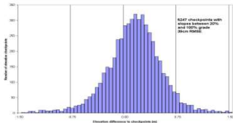
Figure 9. Histogram of the elevation differences between the WorldView-2 stereo satellite elevations for the 25km by 16km area and the 5,247 elevation checkpoints with slopes between 20% and 100% grade. RMSE 39cm.
