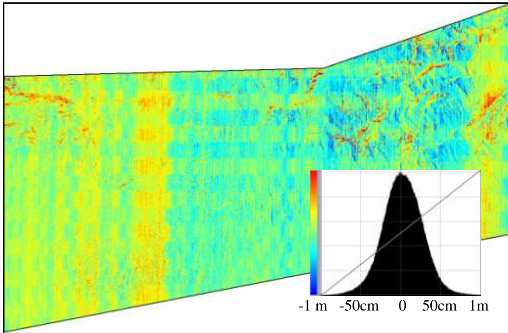
Figure 13. Image of the elevation differences between the GeoEye-1 and LiDAR DEMs displayed as blue for -1m to red for +1m differences. The image and histogram were created in ERMMapper. The standard deviation of the elevation differences is 25cm.
