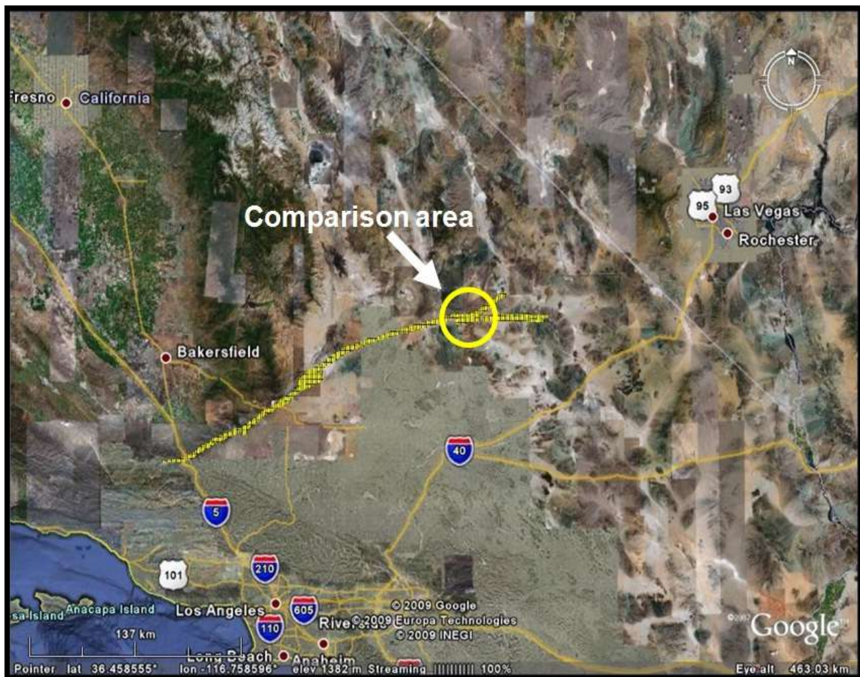
Figure 10. The Garlock Fault OpenTopography LiDAR survey shown on Google Earth. The Garlock Fault LiDAR survey was flown in April 2008. The location of the GeoEye-1 stereo satellite photos, acquired November 30, 2009, is shown by the circle.
