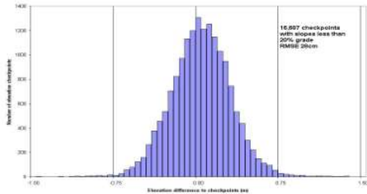
Figure 8. Histogram of the elevation differences between the WorldView-2 stereo satellite elevations for the 25km by 16km area and the 16,687 elevation checkpoints with slopes less than 20% grade. The Guidelines for Digital Elevation Data of the US National Digital Elevation Program (NDEP) recommends that elevation checkpoints should not be chosen in areas with slopes greater than 20% grade. RMSE 28cm.
