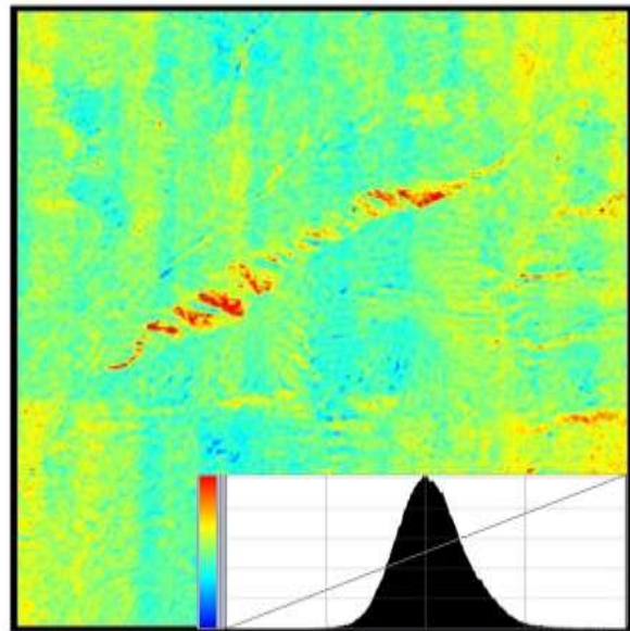
Elevation Differences
