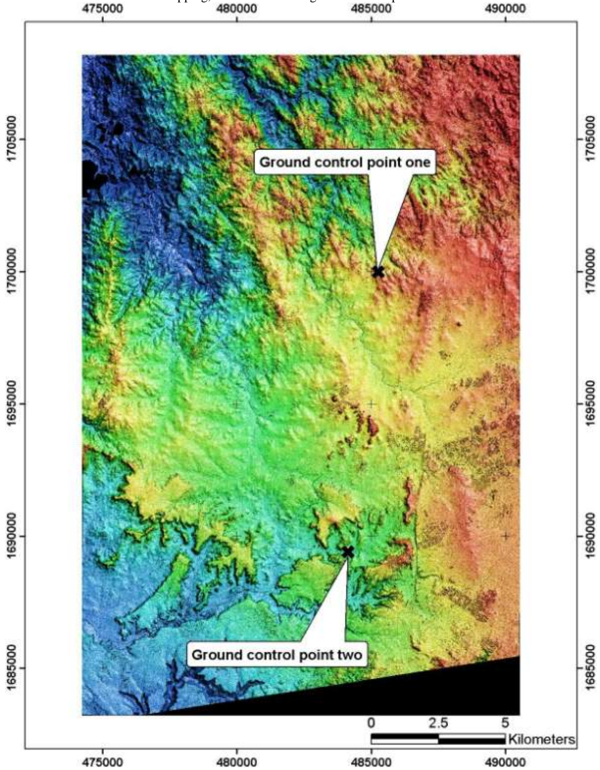
Figure 5. WorldView-2 elevation image created from a 1m posted DEM showing the two ground control points.
