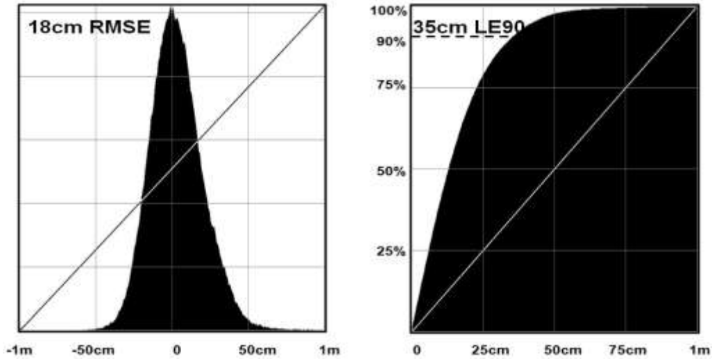
Figure 17. The elevation differences between the GeoEye-1 and LiDAR DEMs for the 500m wide area are shown in a standard histogram on the left and a cumulative histogram on the right. If we assume that the LiDAR DEM is perfect, the GeoEye-1 DEM elevations have an RMSE of 18cm. Ninety percent of the stereo GeoEye elevations are within 35cm of the LiDAR elevations, giving a 90% Linear Error (LE90) of 35cm for this area.
